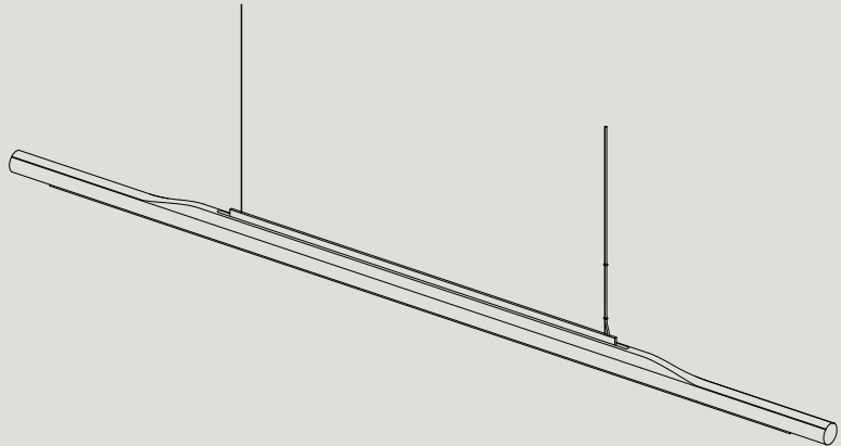
APL L 2200 W 50 H 85 L 86" W 1.9" H 3.4" CEILING CANOPY SPACING L982 / 38.6"
