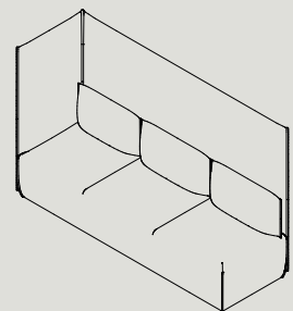
PHA3-R/L* W 2190 D 730 H 1350 S 440 W 86.2" D 28.7" H 53.1" S 17.3"
