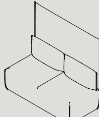
PHB2 W 1460 D 730 H 1350 S 440 W 57.5" D 28.7" H 53.1" S 17.3"
