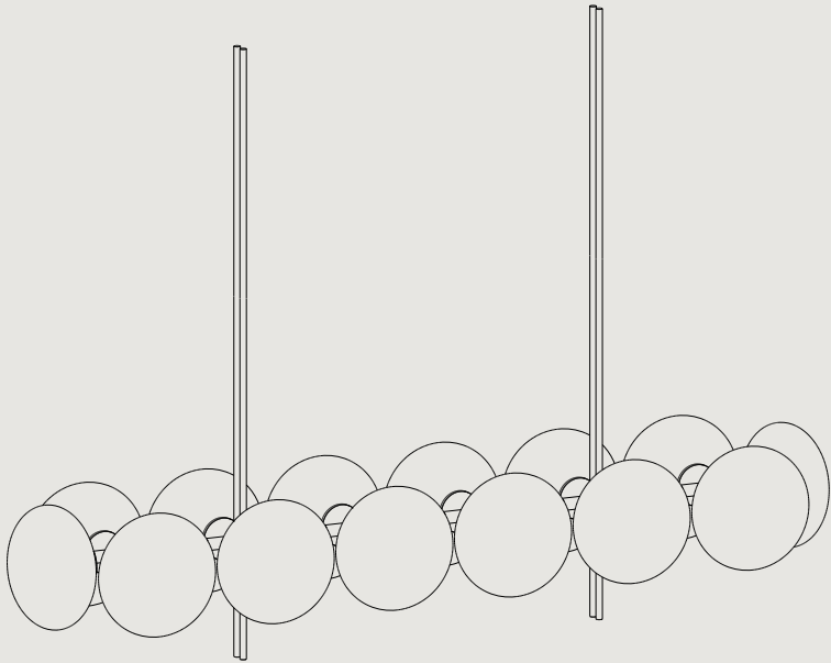
AE214 L 1760 W 460 H 350 L 69.3" W 18.1" H 13.8" MIN DROP HEIGHT - H 600 / 23.6" CEILING CANOPY SPACING L780MM / 30.7"
