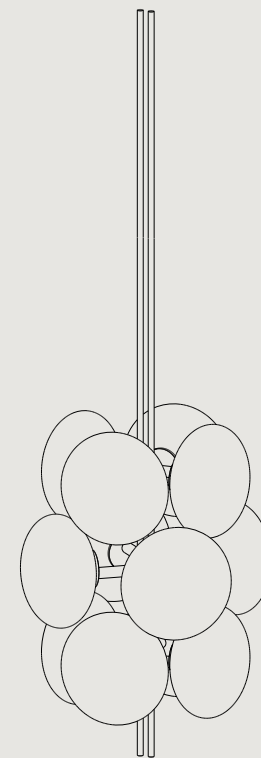
AE112 L 550 W 550 H 740 L 21.7" W 21.7" H 29.1" MIN DROP HEIGHT - H 1,000 / 39.4"
