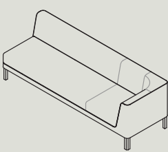
TA3 - R/L* W 2330 D 770 H 725 S400 W 91.7" D 30.3" H 28.5" S 15.7"
