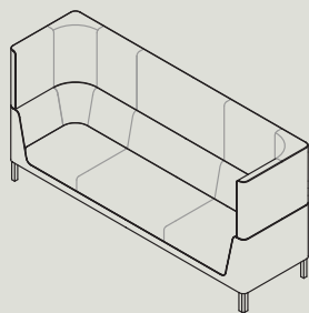
THBL4 W 2700 D 770 H 1300 S 400 W 106.3" D 30.3" H 51.2" S 15.7"
