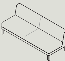
TB3 W 2000 D 770 H 725 S 400 W 78.7" D 30.3" H 28.5" S 15.7"
