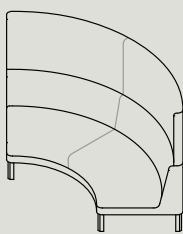
THBB90 W 1575 D 1575 H 1300 IR 750 S 400 W 62.0" D 62.0" H 51.2" IR 29.5" S 15.7"
