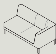
TA1 - R/L* W 1530 D 770 H 725 S400 W 60.2" D 30.3" H 28.5" S 15.7"
