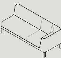
TA2 - R/L* W 1930 D 770 H 725 S400 W 75.0" D 30.3" H 28.5" S 15.7"
