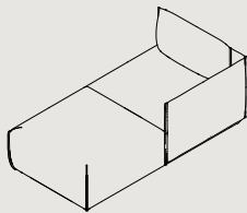
HCH-1-R/L* W 910 D 1740 H 750 S 410
