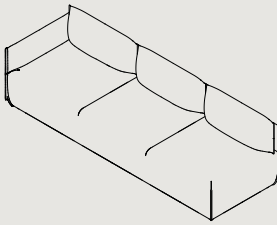
HA3-R/L* W 2570 D 910 H 750 S 410
