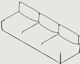
HB3 W 2490 D 910 H 750 S 410
