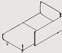
HCH-1.5-R/L-LOFT* W 910 D 1740 H 750 S 410
