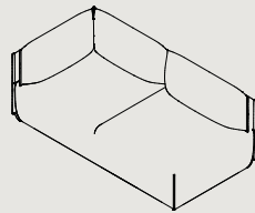
HCA2-R/L* W 1740 D 910 H 750 S 410
