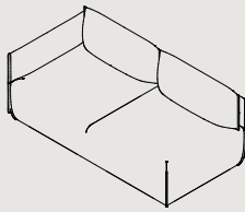
HA2-R/L* W 1740 D 910 H 750 S 410
