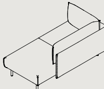
HCHC-1.5-R/L-LOFT* W 910 D 1740 H 750 S 410
