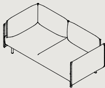
HCL2-R/L-LOFT* W 1820 D 910 H 750 S 410
