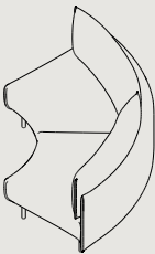
HB45D-LOFT W 1725 D 1725 H 750 S 410 IN Ø1700 / OUT Ø3520
